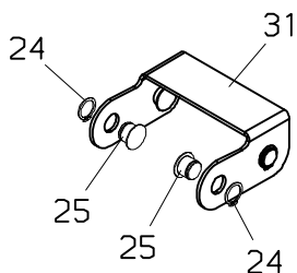
Schubarm 4 Boom extension 4 Extension 4
