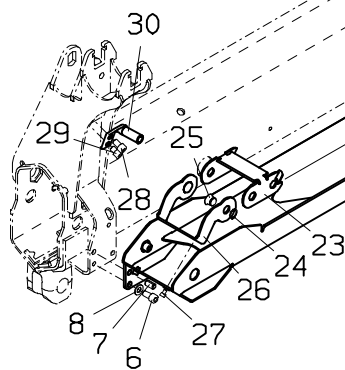
Schubarm 4 Boom extension 4 Extension 4
